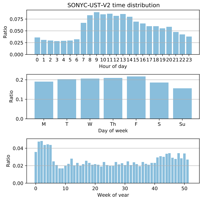
Figure 5: Distribution of dataset recordings per hour of the day, day of the week, and week of the year.
