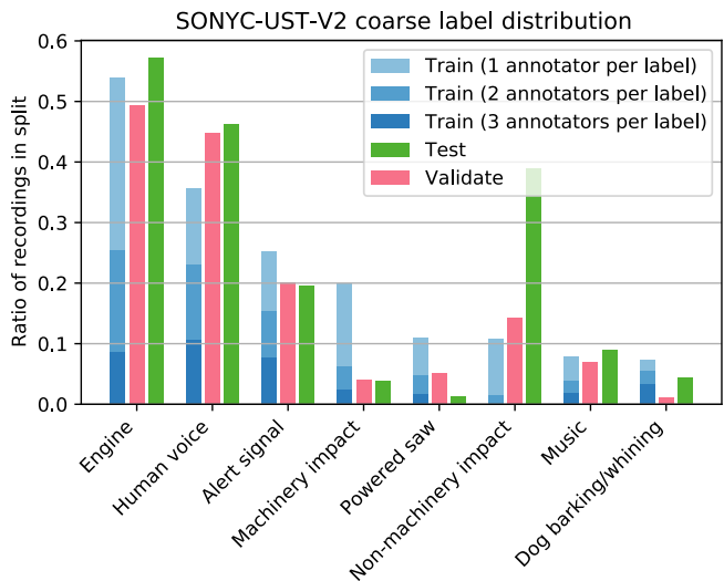
Figure 4: SONYC-UST tag distribution normalized for each recording split, in decreasing order of frequency in the training split. The shades of blue indicate how many annotators tagged the class in a training set recording, i.e., darker shades of blue indicate higher annotator agreement.
