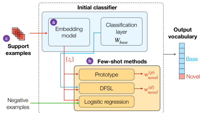
Figure 1: Few-shot continual learning framework for multi-label audio classification. We analyze (a) embedding model architectures, (b) few-shot methods, and (c) support set selection.
